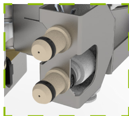
Hydraulic connection without Americano (Original E'line)
