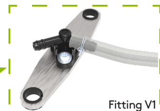
Fitting V1 Without crema nozzle Silicon tube
